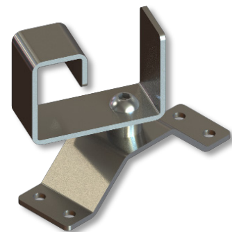
RT-RHLS REAR HANDLE LOCK (SHORT BASE)
