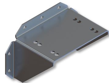
RT-47200 UNIVERSAL ALUMINIUM MOUNTING SHELF FOR ROLL-RITE ARM(S)
