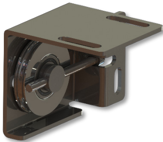
R.DS COMPLETE COMPACT REAR ADJUSTER (DRIVERS SIDE)
