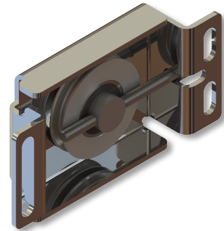
R.SW COMPLETE BI-DIRECTIONAL REAR ADJUSTER
