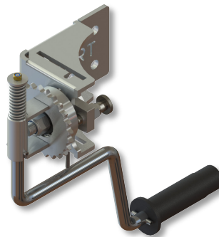
HT-CHD COMPLETE CHAIN DRIVE HANDLE ASSEMBLY
