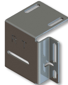
HT-RA003EXT PASSENGER SIDE EXTENDED ADJUSTER BRACKET (STAINLESS)
