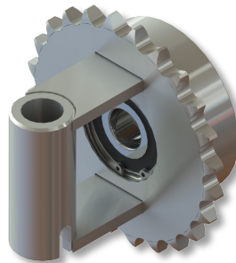
HT-HAB003/C STEEL CHAIN DRIVE SPROCKET
