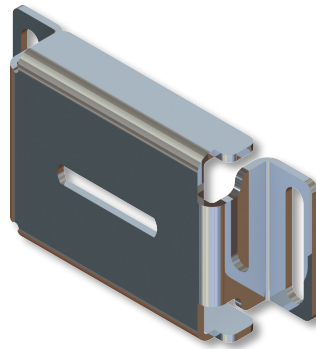
HT-RA005 BI-DIRECTIONAL ADJUSTER BRACKET (STAINLESS)
