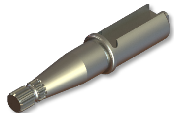
RT-STL15 ROLL TUBE TO UNI JOINT SPLINE ADAPTOR (15 TOOTH)
