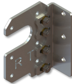
RT-21100 HOLLOWSHAFT MOUNTING BRACKET
