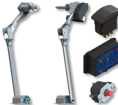
RT-DAE2 (S/R) DUAL ARM ELECTRIC KIT C/W MOTOR, ADAPTOR & HARDWIRED CONTROLLER
