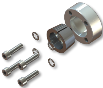
HT-SSDSTLA0 COMPLETE TAPER LOCK ASSEMBLY (COMES WITH MOUNTING SCREWS)
