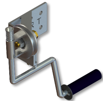
HT-HAB BELT DRIVE HANDLE ASSEMBLY
