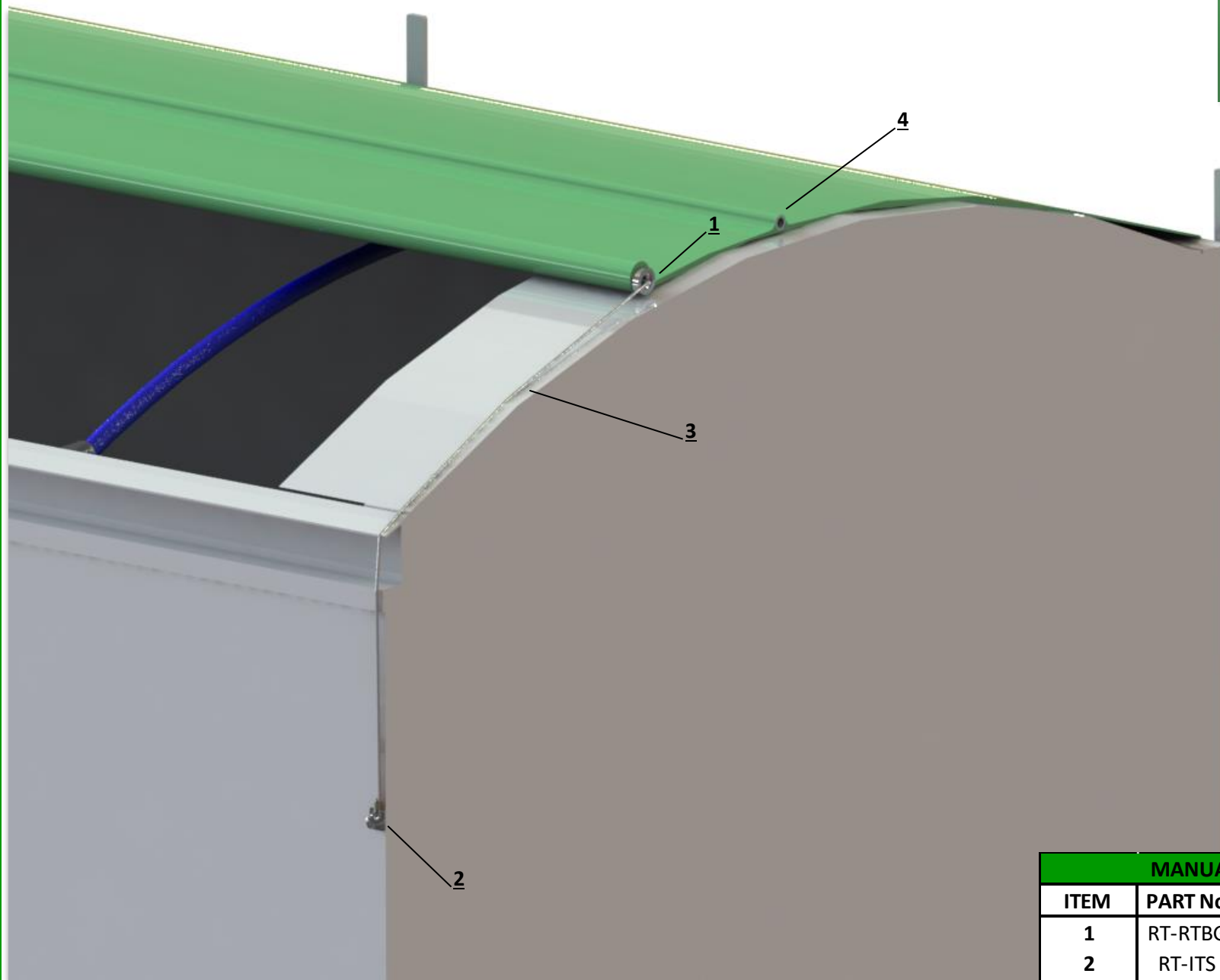
RT-ITS INNER TENSION SPRING KIT c/w cable
